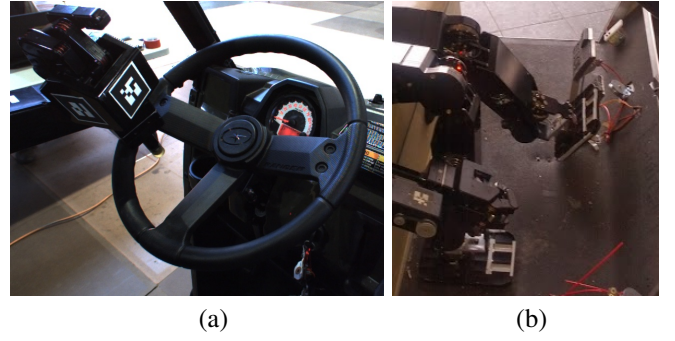
Fig. 7. (a) Peg-in-wheel method for steering (Polaris); (b) Foot arrangement for pedal control (Club Car)
