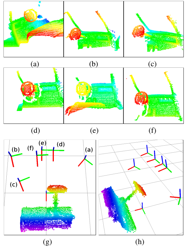
Fig. 8. Club Car dashboard registration for sensor head pose estimation. (a-f) Hokuyo point clouds acquired from different poses, in sensor_head frame; (g, h) Views of estimated sensor head locations with respect to the dashboard reference cloud and origin (all point clouds colored by X , grid squares are 1 m)
