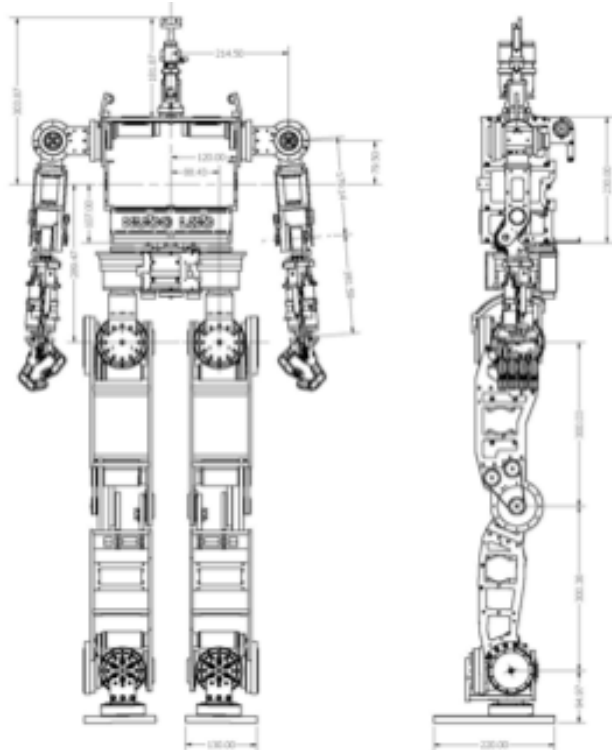
Figure 1: Hubo Schematic
