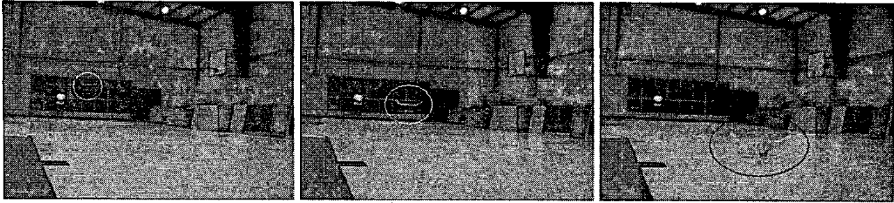
Figure 11: The optic flow on the basketball gym floor is kept constant by the control system. That is, the aircraft (encircled) forward velocity is decreased in proportion with its altitude to land smoothly. Left: Aircraft just after hand launch. Middle: Aircraft midway through landing sequence at proportionally lower altitude and velocity. Right: Aircraft comes to a smooth landing within 25 meters from starting point.
