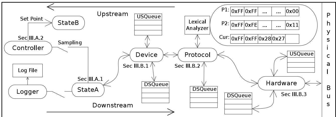
Fig. 1. Schematic of the data flow through the Conductor system. Data enters at either the State or Hardware level traveling downstream or upstream respectively. At each level the requests are cached and concentrated as appropriate to make efficient usage of bus resources. Each component in the system is tagged with its section number in the paper, for easy reference.
