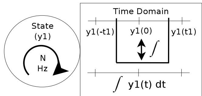
Fig. 2. The State acts as a gatekeeper to a number of computationally useful tools including the quantity's history, integral, and derivative.
