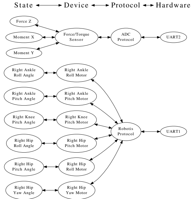
Fig. 7. An illustration of the node arrangement in the example system, shows the topology for implementing the right leg controller of mini-Hubo.
