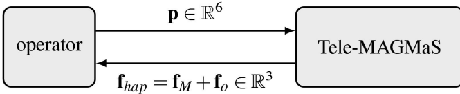
Fig. 4: Illustration of the bilateral tele-operation scheme, with operator commanding the position \mathbf{p} and receiving a force feedback \mathbf{f}_{hap} rendering the system inertia and proximity to obstacles.
